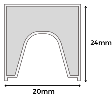
TOP RAIL
