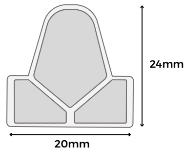
BOTTOM RAIL
